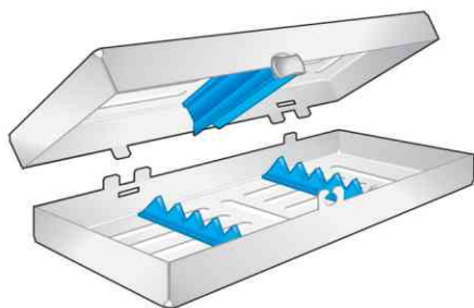
BD-2490 185 x 75 x 35 mm For 5 Instruments
